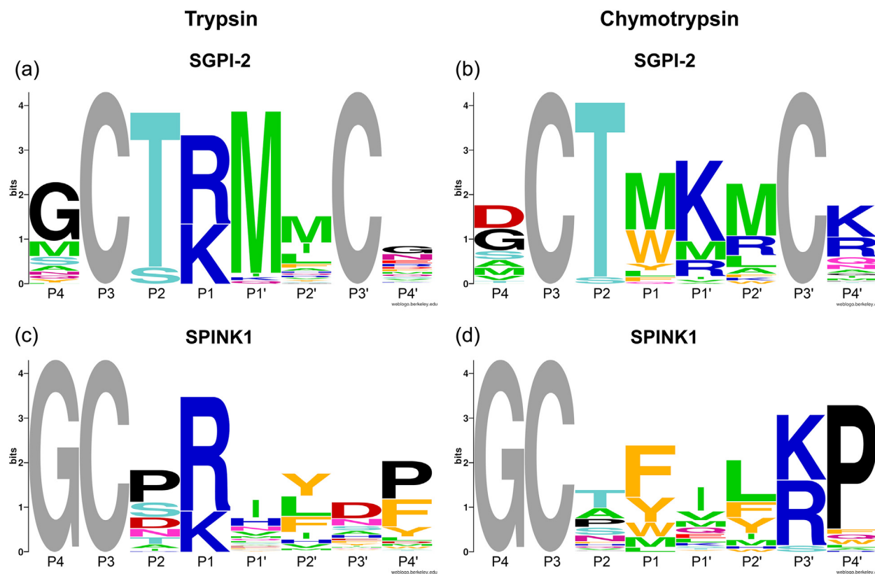
Fig. 2. Sequence logos generated by the WebLogo program representing the P4–P4' positions of the phage display-selected inhibitors. Sequence logo representation of (a) bovine trypsin-selected SGPI-2 variants, (b) bovine chymotrypsin-selected SGPI-2 variants, (c) bovine trypsin-selected SPINK1 variants and (d) bovine chymotrypsin-selected SPINK1 variants. Amino acids are represented by their one letter code. The overall height of a stack of letters indicates the degree of conservation. Individual symbol height shows the codon-normalized relative frequency of the residue. Maximal symbol height corresponds to completely conserved amino acids, that is, Cys residues and the P4 Gly in SPINK1 shown in gray.
